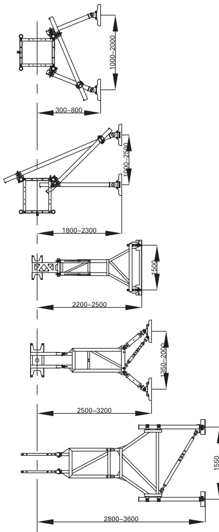
Mast tie
