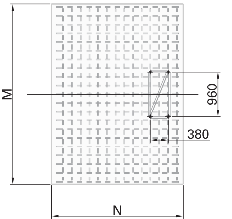
Foundation
